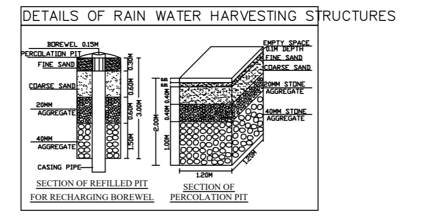
DETAILS OF RAIN WATER HARVESTING STRUCTURES
